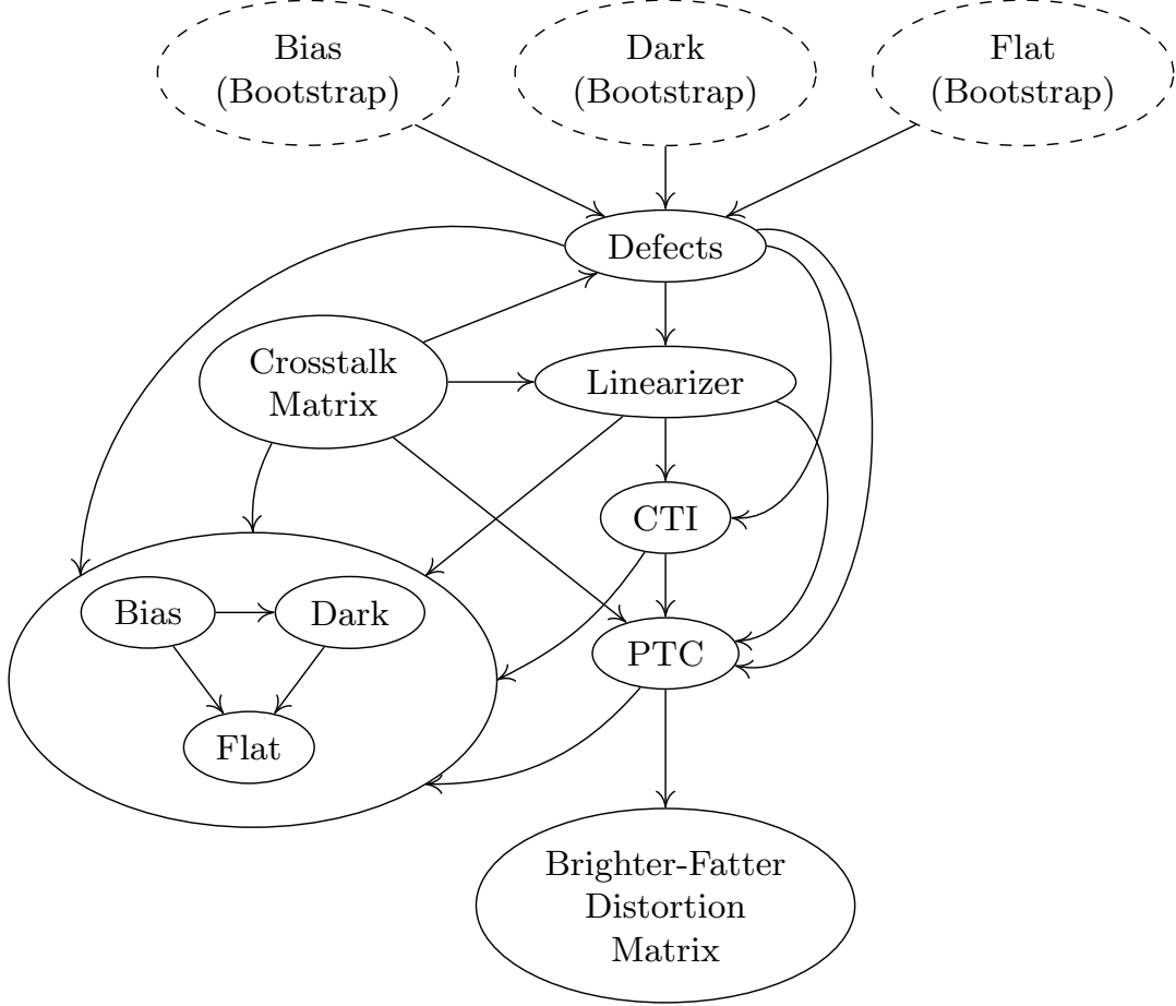
Figure 2. Calibration production dependency graph. Arrows indicate data or dependency flow ("x \rightarrow y" means "y depends on x"). Solid outlined boxes represent datasets that are deployed/released with data products while dashed boxes represent internal or intermediate datasets that are not formally released to users.
