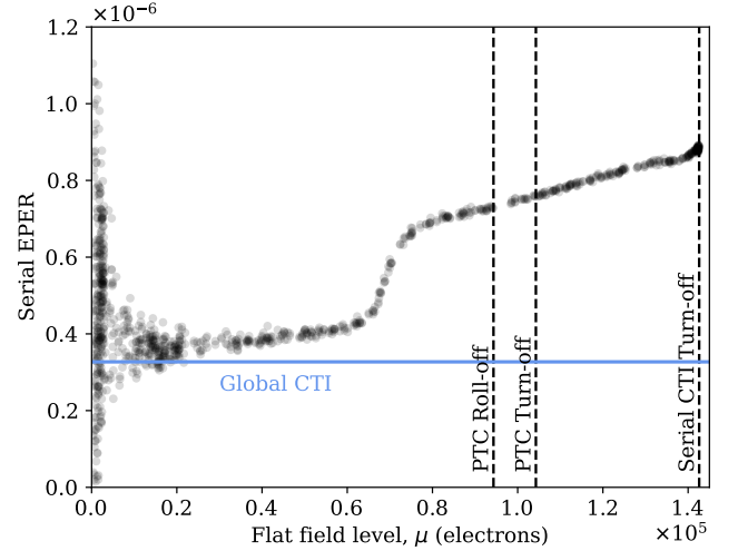
Figure 6. Serial EPER statistics as a function of flat-field signal level for detector/amplifier R22-S10/C04. Vertical markers indicate the PTC rolloff and turnoff thresholds (described in §5.7) and the serial CTI turnoff derived from the low-signal trend. The global CTI fit produces the overall offset of the measured curve at all signal levels.
