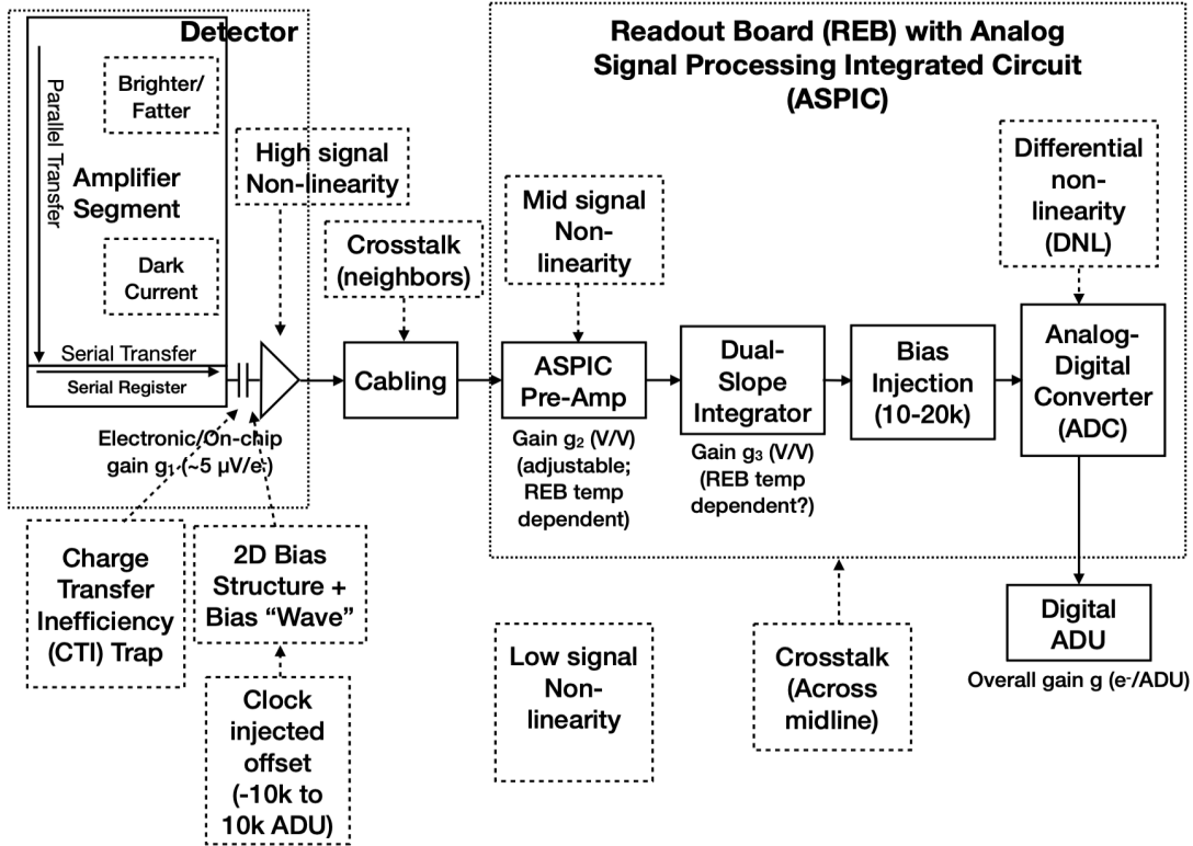
Figure 4. Photon transfer and data-acquisition model for the LSSTCam detectors and electronic readout board (REB). Instrumental effects seen in images are shown as dashed boxes; arrows indicate where each effect enters the chain. Low-signal nonlinearities in LSSTCam’s detector response have been observed, but their origin is not yet established; that contribution appears as a disconnected box.
