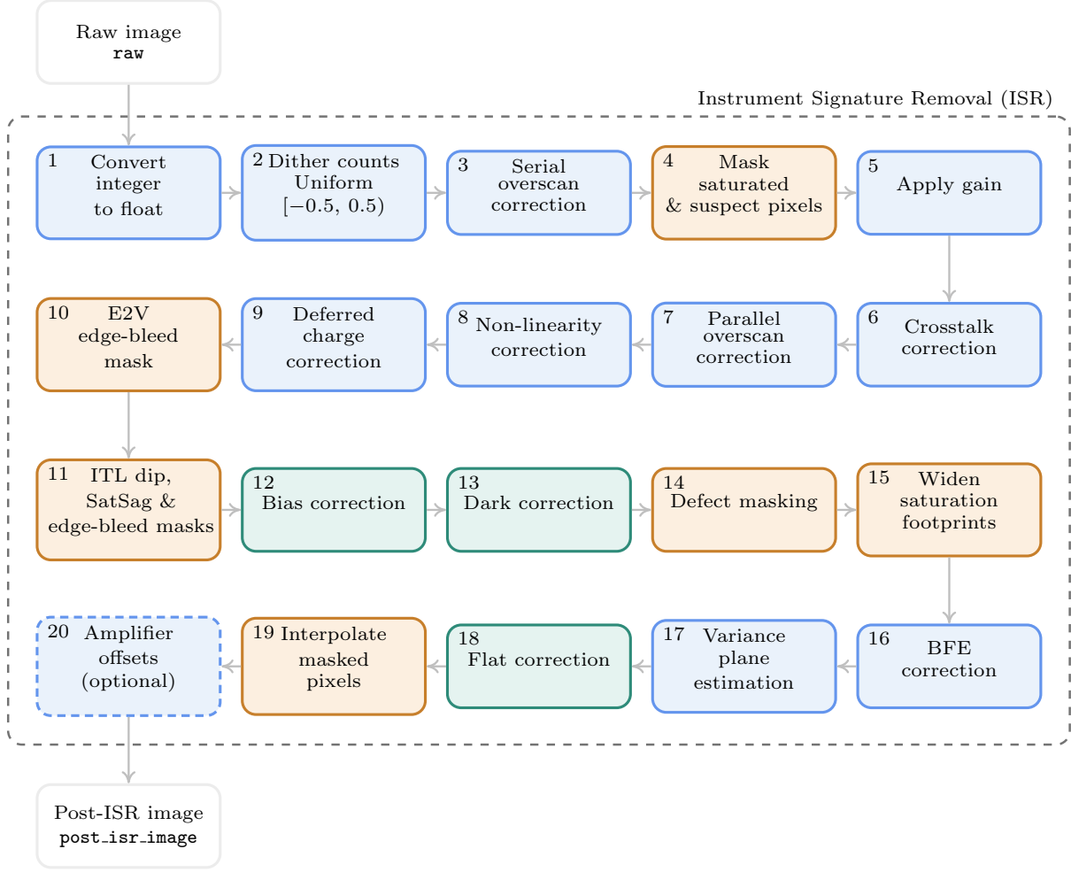
Figure 10. Outline of the Instrument Signature Removal Pipeline (ISR) applied to LSSTCam science images for DP2. The steps in the pipeline follow a very specific sequence determined by the physics of the instrument signature and where it enters in the photon transfer chain.
