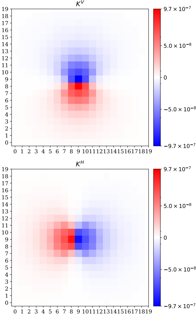
Figure 14. Example BFE correction kernels K^V (vertical) and K^H (horizontal) derived from the electrostatic BFE model for amplifier C03 on LSSTCam detector 94. The diverging color scale shows the fractional charge redistributed across pixel boundaries; each kernel sums to zero to conserve charge and exhibits the antisymmetric dipole structure that moves flux from the brighter pixel to its neighbors.
