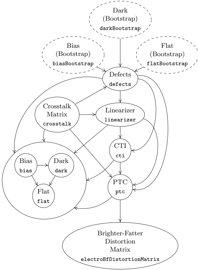
Figure 6. Calibration production dependency graph. Arrows indicate data or dependency flow (“ x \rightarrow y ” means “ y depends on x ”). Solid outlined boxes represent datasets that are deployed/released with data products while dashed boxes represent internal or intermediate datasets that are not formally released to users.
